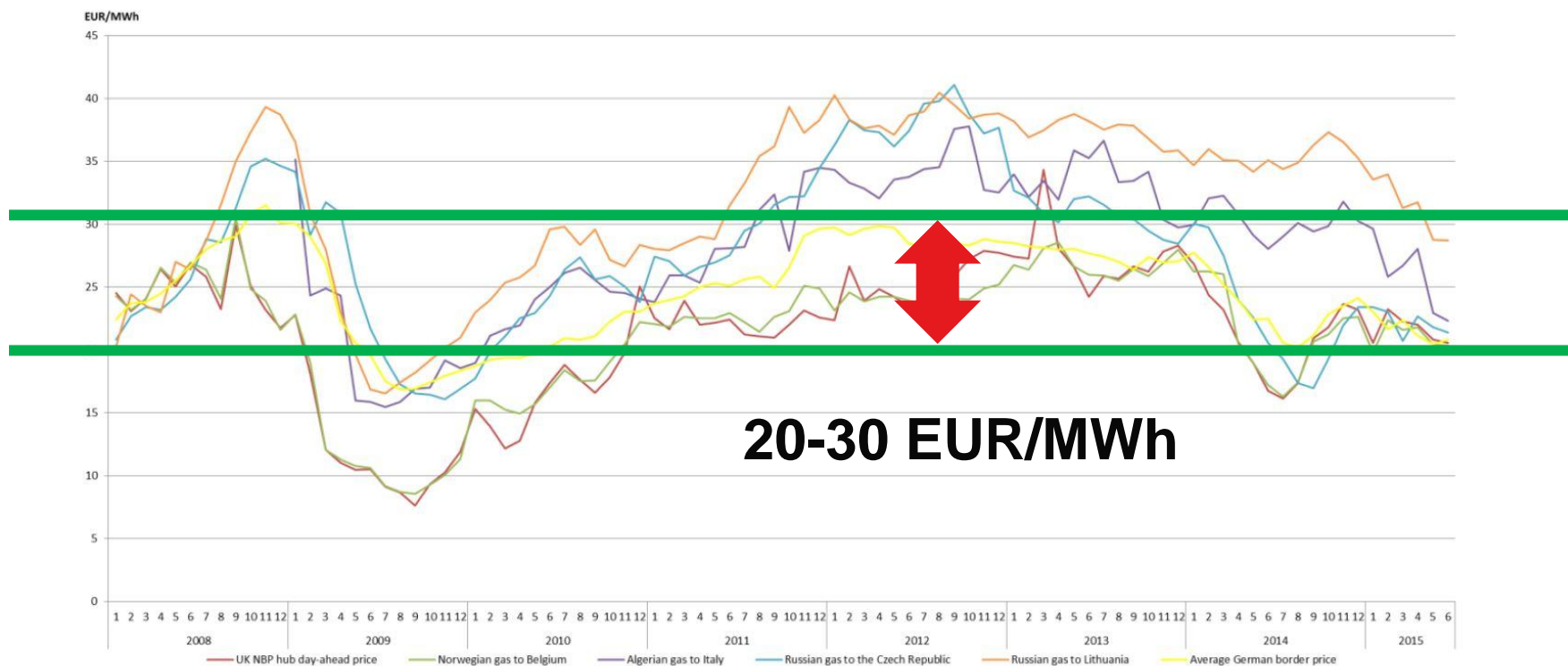
Figure 21. Comparison of EU wholesale gas price estimations
