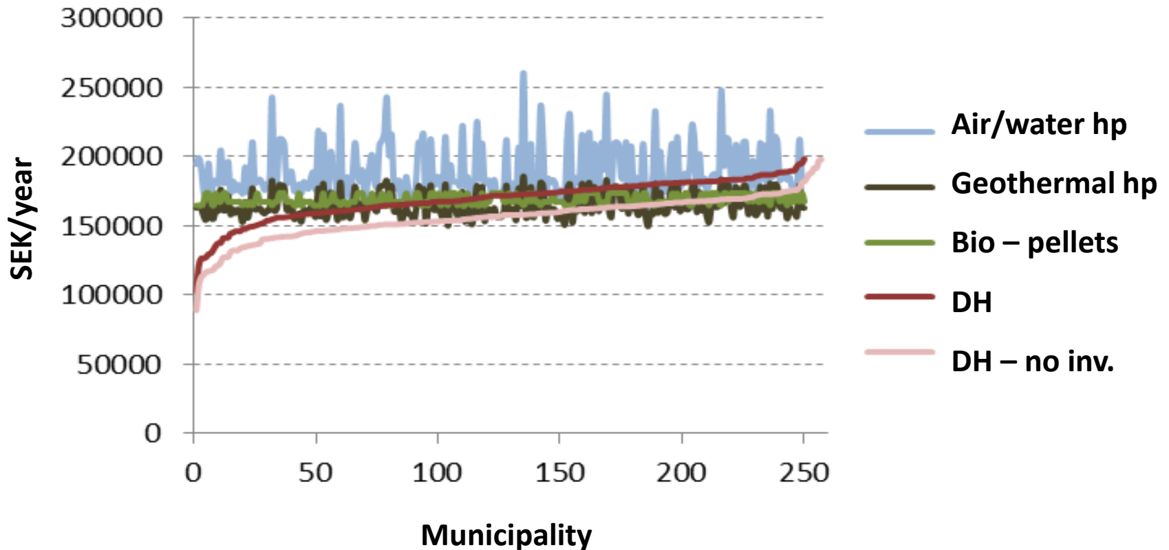
Cost for heating a small multifamily house in Swedish municipalities
